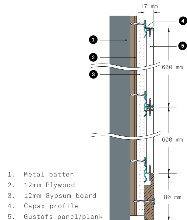
PARTITION WALL CONSTRUCTION 17+24mm
