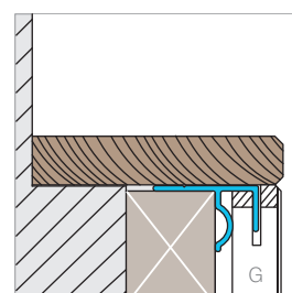
COVER PROFILE 140x16mm
