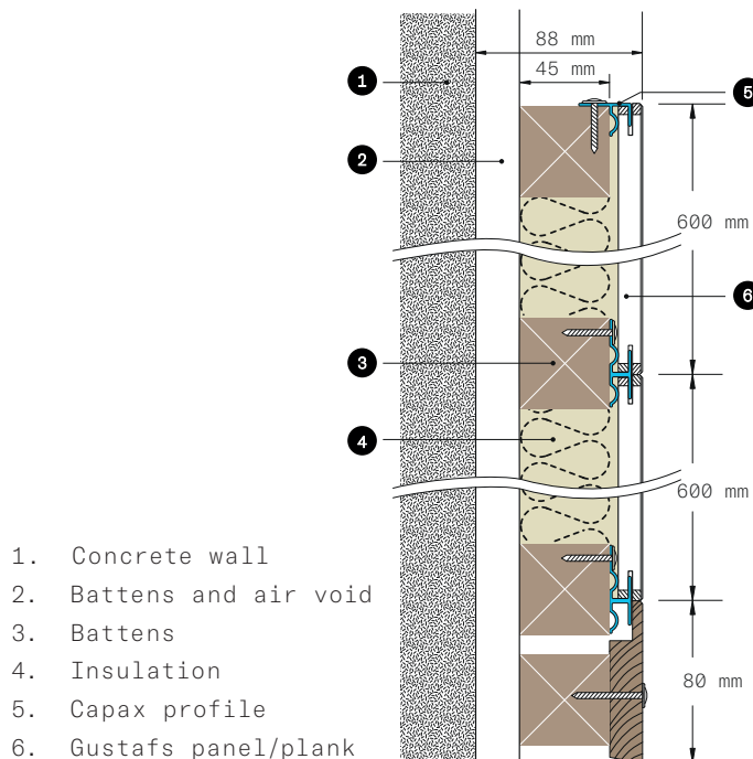
ACOUSTIC CONSTRUCTION 88mm
