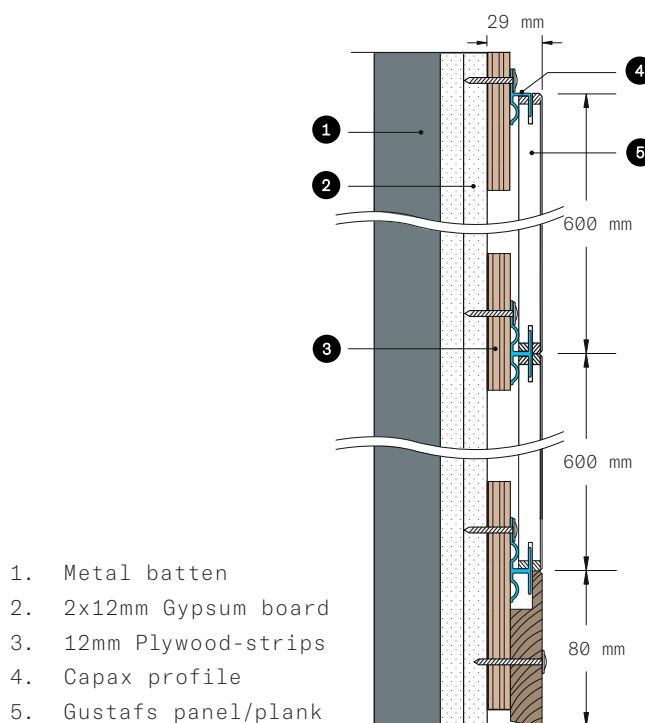
WALL ASSEMBLY 29+24mm
