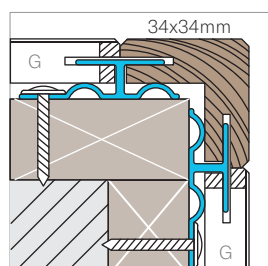
CORNER PROFILE 34x34mm
