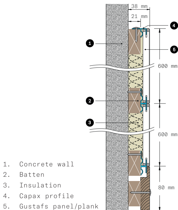
ACOUSTIC CONSTRUCTION 38mm
