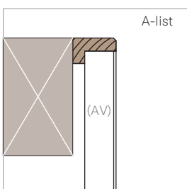
A-EDGE COVER 18x10mm
